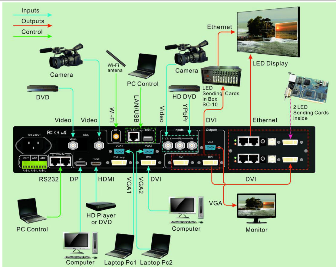
Connection diagram
