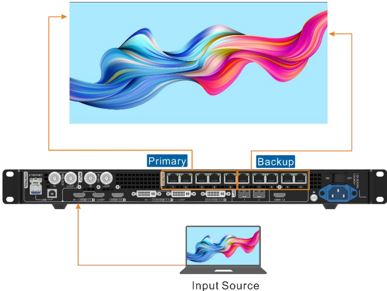
Figure 5-27 Ethernet port backup connection
