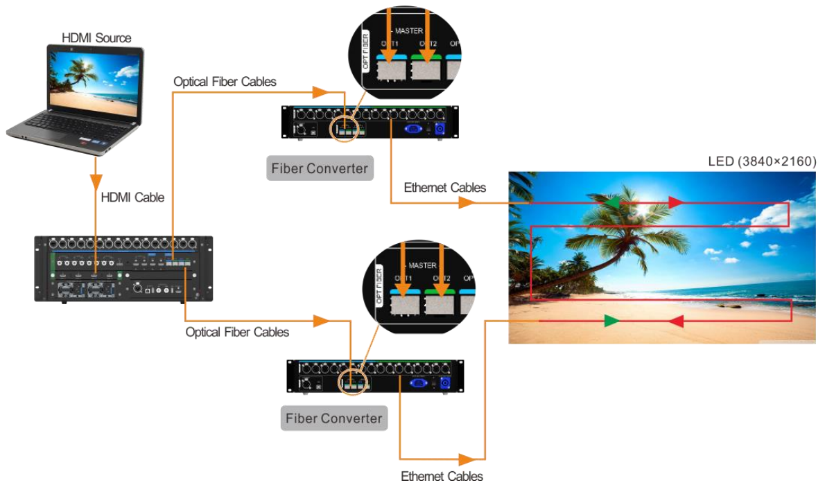
Figure 7-28 Connections for copy mode
