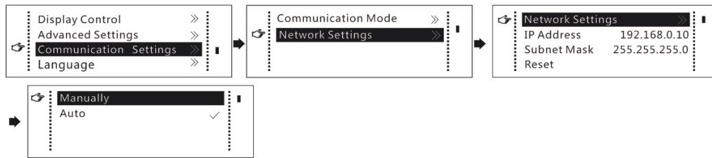
Figure 6-14 Network settings
